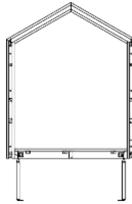
K-K ( 1/50 )
